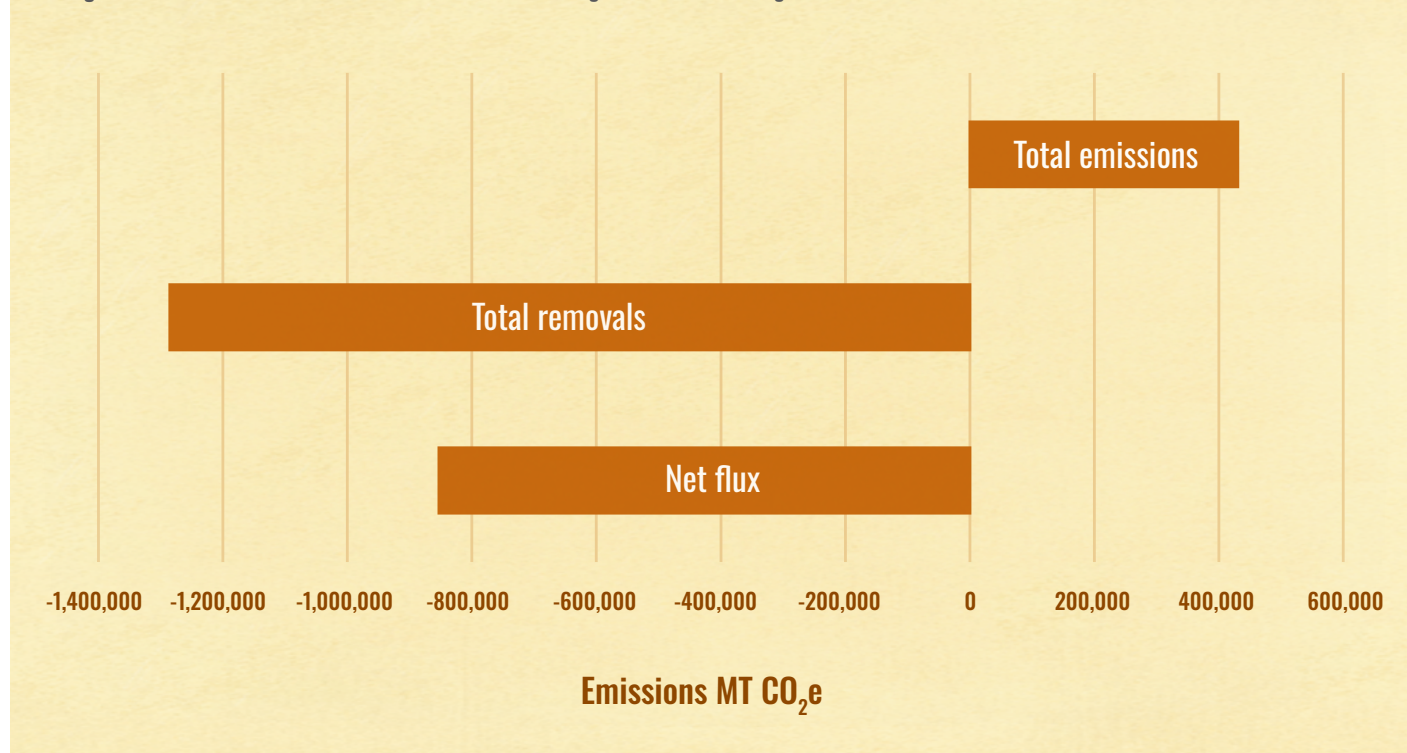
Figure 33: Carbon emissions and removals from natural and working lands in the DRCOG region in 2022.
